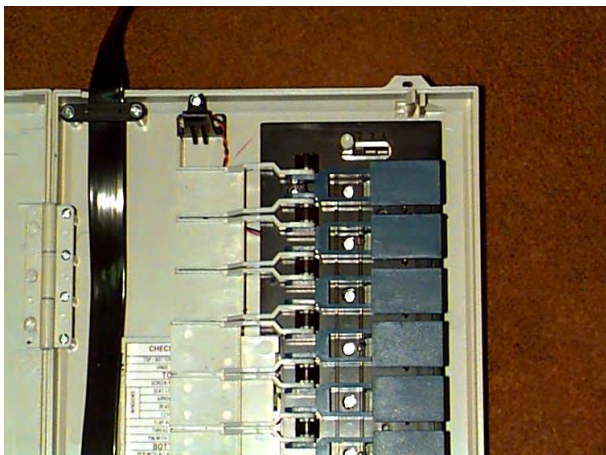
Fig. 11.3: Masking Ballot Buttons
