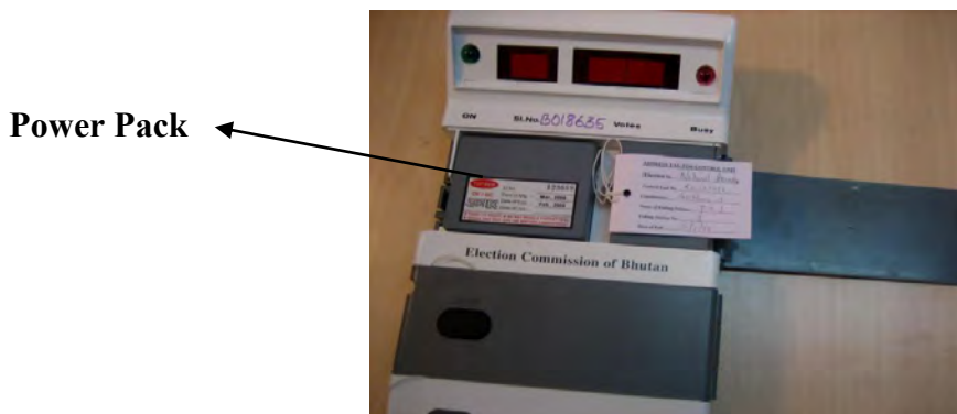
Fig. 11.8: Power Pack Installation
