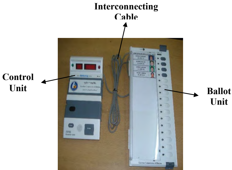
Fig. 10.1: The Electronic Voting Machine
